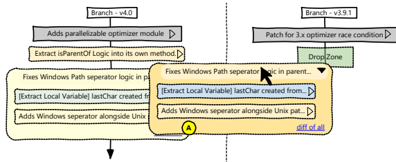
Fig. 3. Commit bubbles are copied from one branch and integrated into another by drag-and-dropping the commit bubble from the source branch to the target branch. While existing tools optimize for making commits, our tool makes revising history tasks just as easy.
